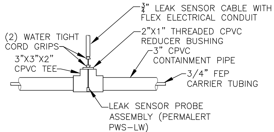
LEAK SENSOR INSTALLATION DETAIL N.T.S.
