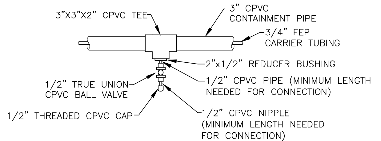
DRAIN INSTALLATION DETAIL N.T.S.
