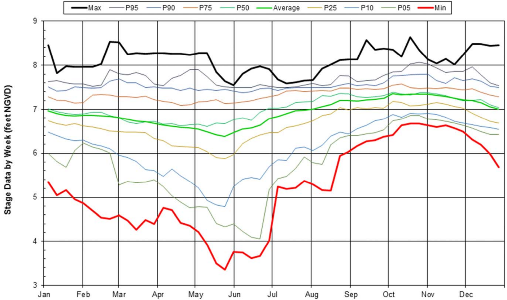
FIGURE 2 Cyclic Analysis of S333_T Daily Stage Data (2012-2018) by Week
