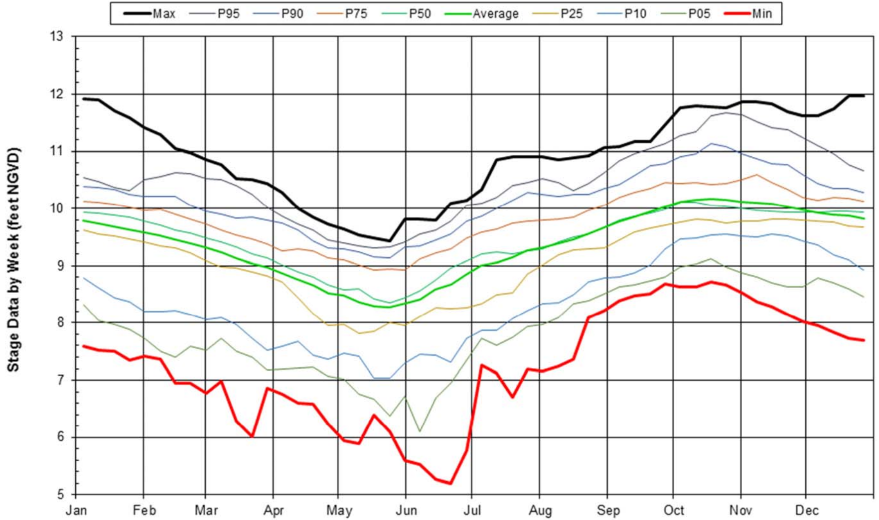
FIGURE 1 Cyclic Analysis of S333_H Daily Stage Data (2012-2018) by Week
